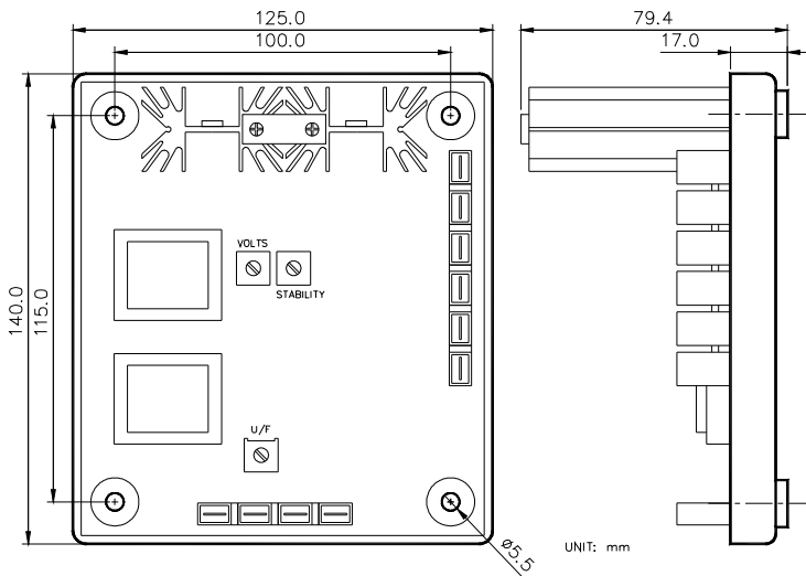
Outline Drawing Figure 3
