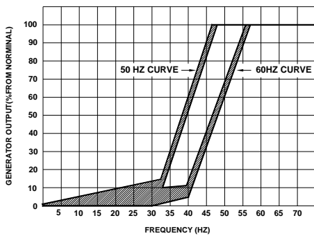
Figure 1 Frequency Compensation Curves
