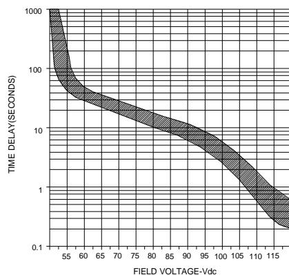
Figure 2 Typical Time Delay Characteristic Curve
