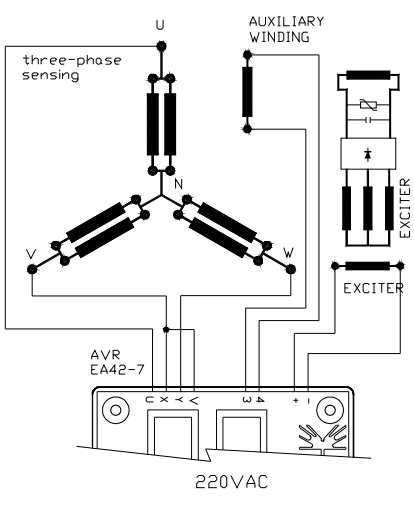
Wiring Diagram Figure 5
